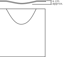
60X120 Bag* 59,55x119,30 cm - 23.45"x46.96" 60X60 Bag* 59,55x59,55 cm - 23.45"x23.45" 30X60 Bag* 29,75x59,55 cm - 11.71"x23.45"
